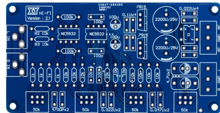
Blind Hole PCB
