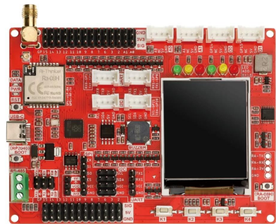
RP2040 LoRaWAN RA-08H Development Board(868Mhz/915Mhz)
